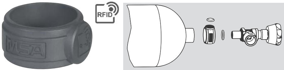
RFID Holder Rings , pack of 10, for \varnothing 34–40 mm, composite cylinders (10128846) RFID Holder Rings , pack of 10, for \varnothing 26–30 mm, steel cylinders (10146101)
